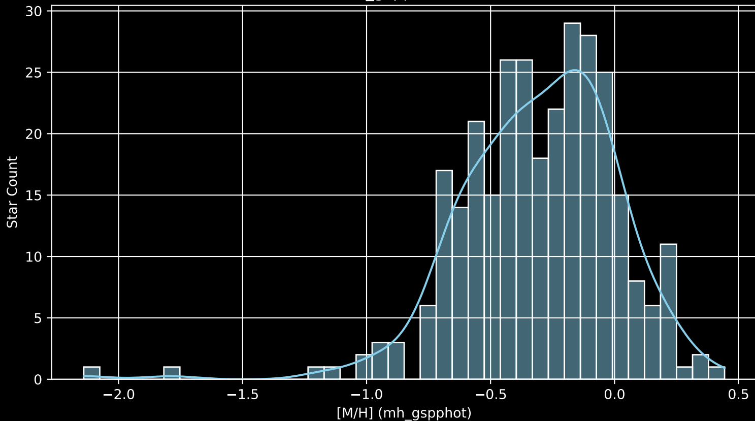
GALAH DR4 Field: [6892] [M/H] (mh_gspphot) (n= 303)
