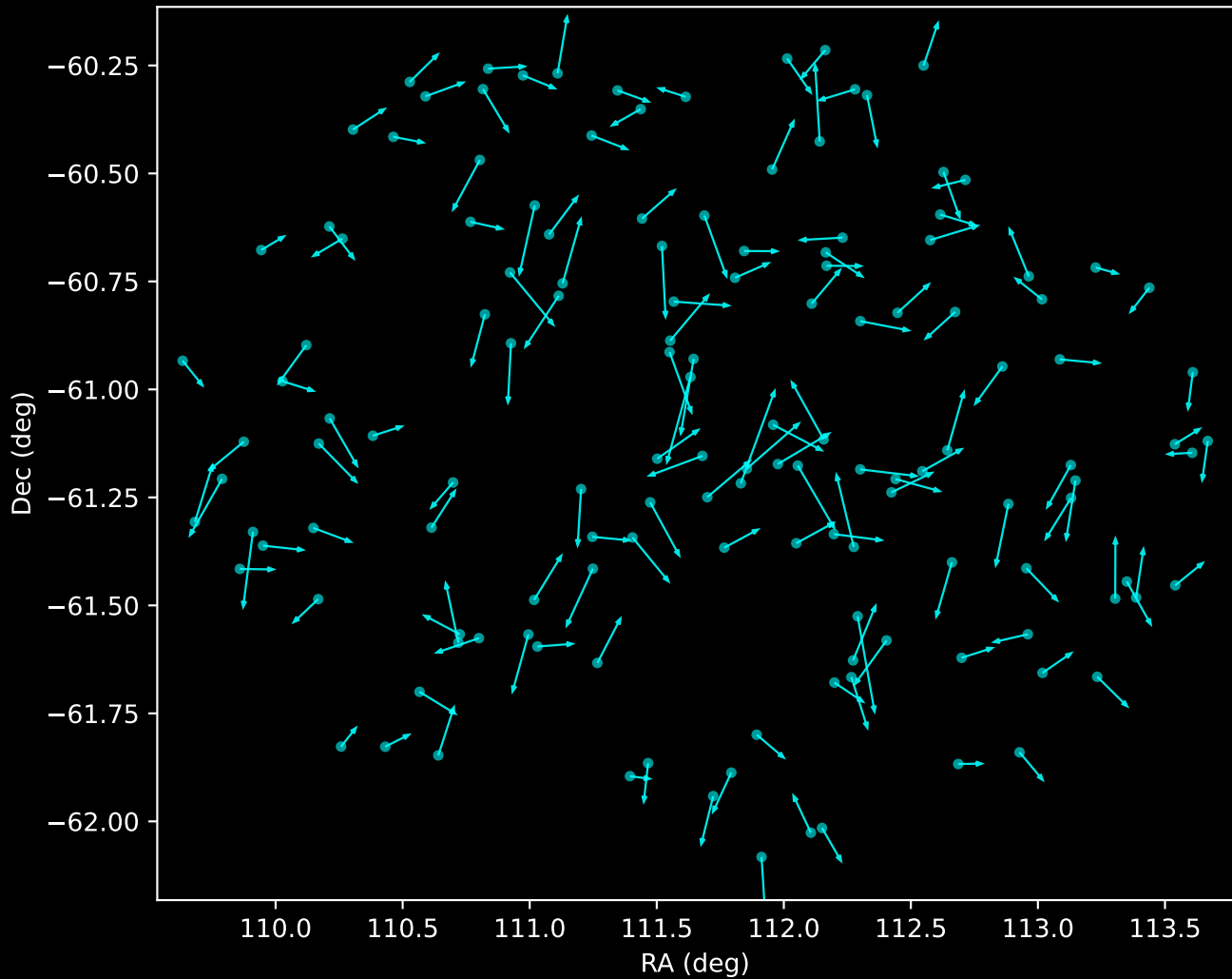
GALAH DR4 Noise Stream Proper Motion Vectors (n=141)
