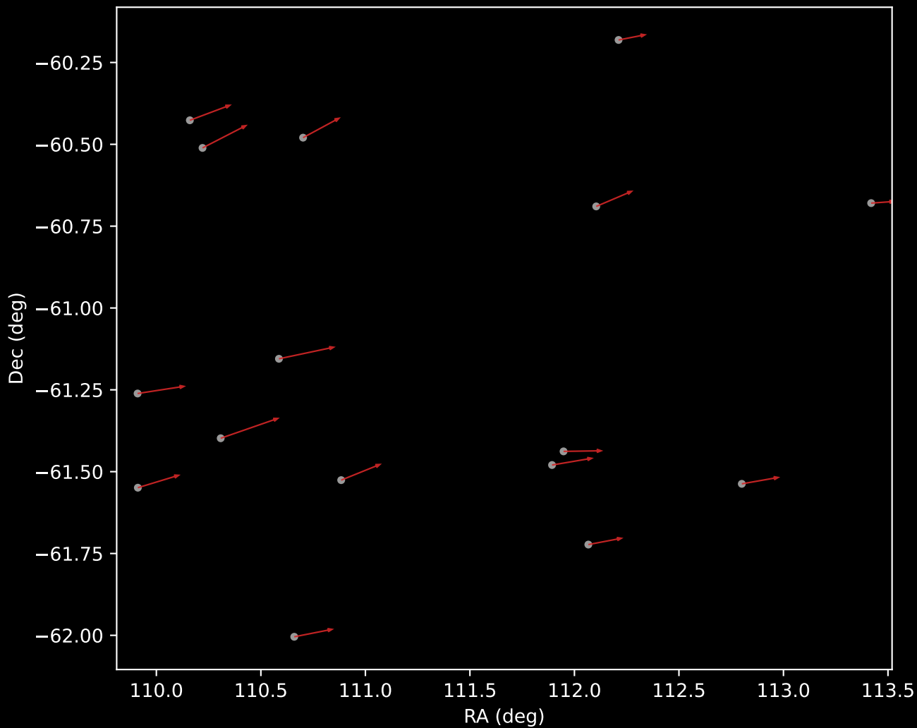
GALAH DR4 Cluster 6 Proper Motion Vectors (n=16)
