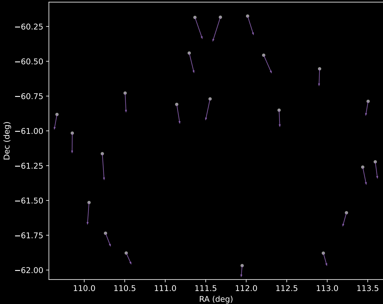
GALAH DR4 Cluster 8 Proper Motion Vectors (n=22)
