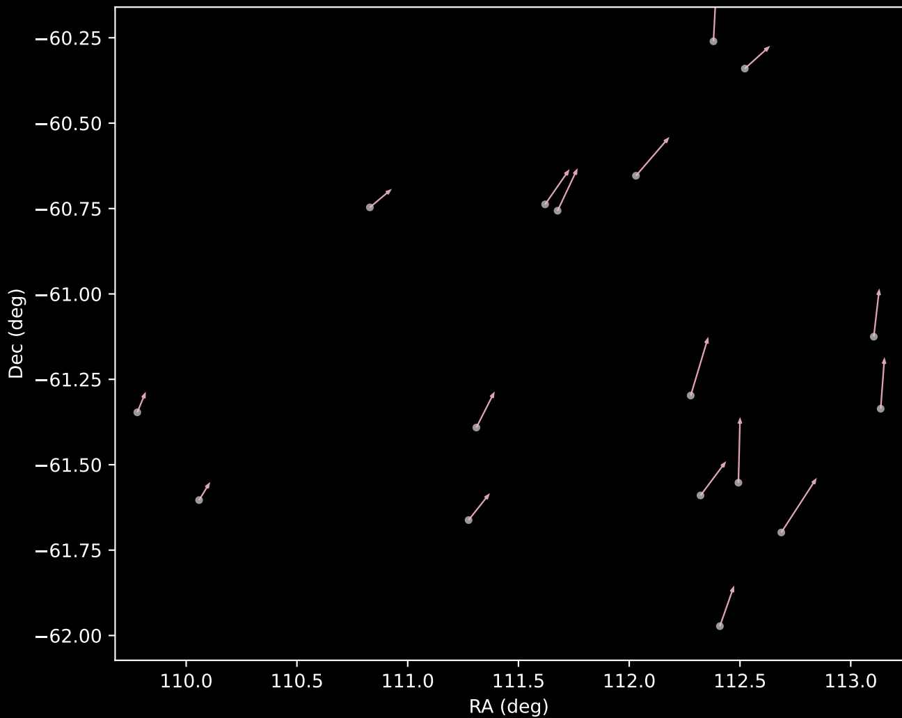
GALAH DR4 Cluster 13 Proper Motion Vectors (n=17)
