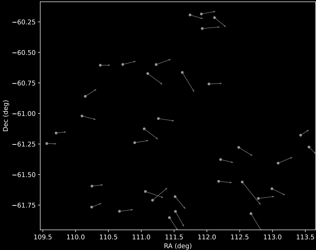
GALAH DR4 Cluster 14 Proper Motion Vectors (n=35)
