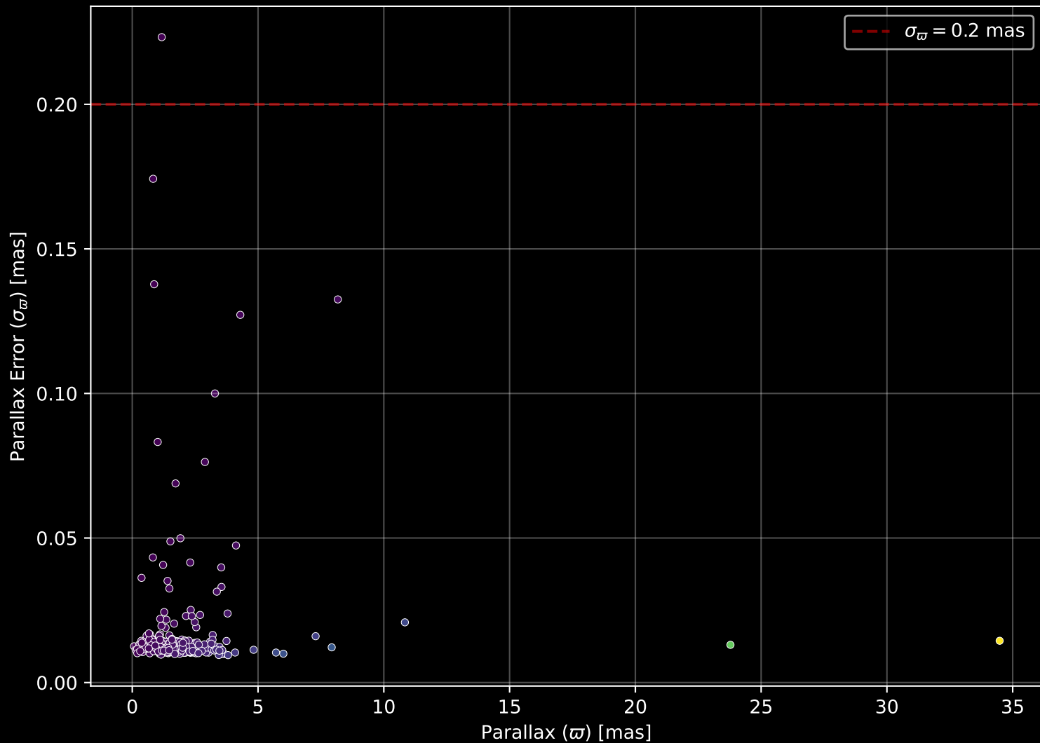
GALAH DR4 Field: [6892] Parallax Quality (n= 303)
