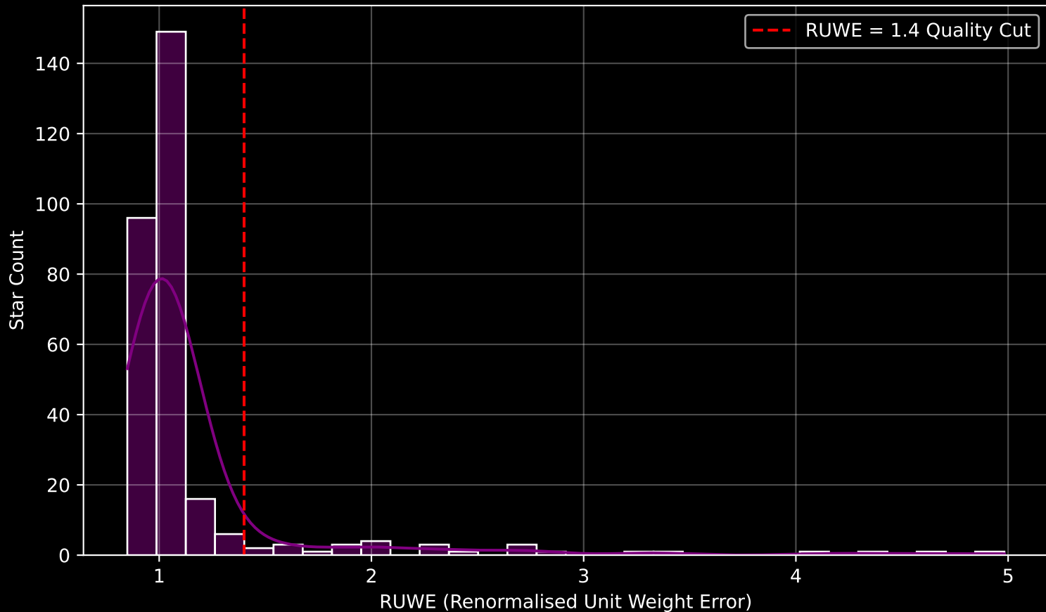
GALAH DR4 Field [6892] RUWE Distribution (n= 294)
