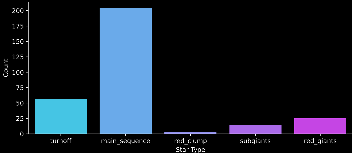
GALAH DR4 Field: [6892] Count plot of Star Type
