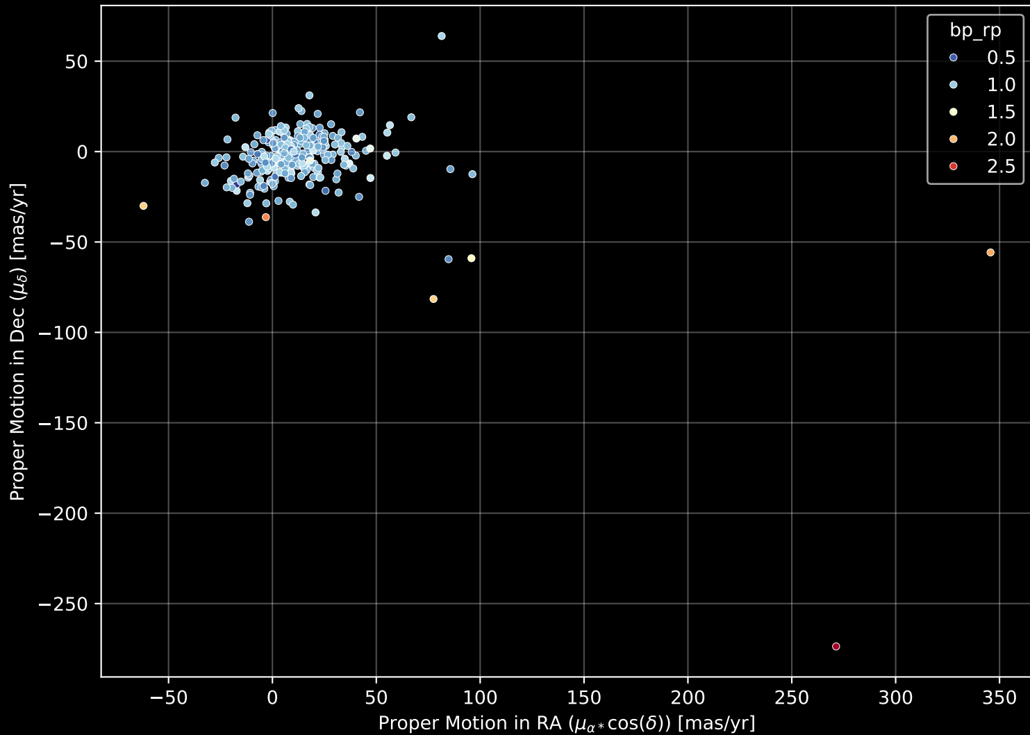
GALAH DR4 Field: [6892] Proper Motion Diagram (n= 303)
